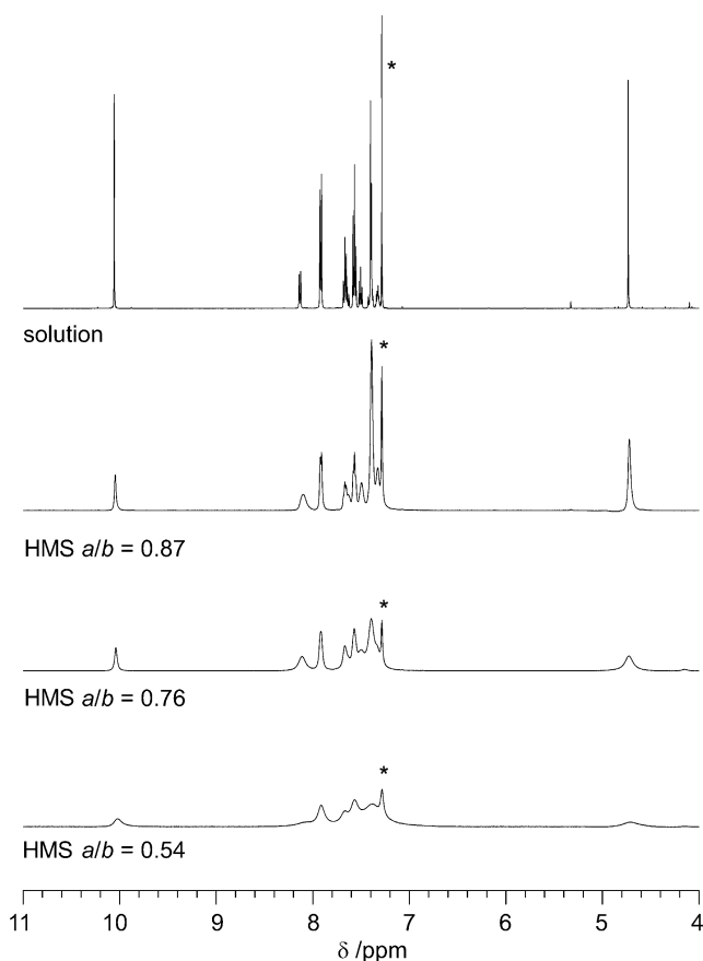
Figure 3. Top: Solution-state ^1\text{H} NMR spectrum of 5 mM benzoic acid, benzaldehyde and benzyl alcohol in \text{CDCl}_3 . Other traces: same mixture in the presence of silica HMS with variable shell thickness and a/b ratios. All the traces are normalized by the area of the peak at 10 ppm. The line width of residual \text{CHCl}_3 (asterisk) in the sample with a/b = 0.87 is about 6 Hz. Different signals within the same spectrum exhibit different linewidths depending on the affinity of the parent molecules for the silica.
