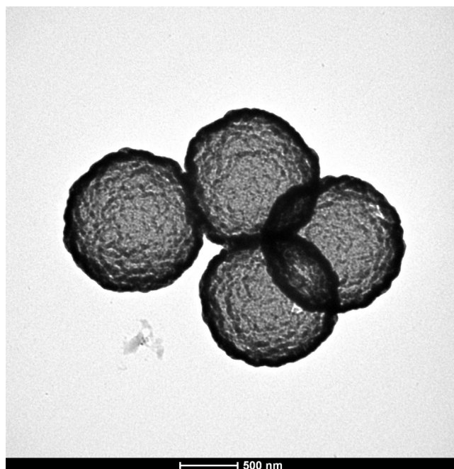
Figure 2. Representative TEM image of silica hollow microspheres prepared as described in the text. The estimated shell thickness is about 75 nm and the average diameter is about 1200 nm ( a/b = 0.87 ).
