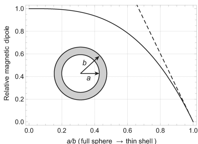
Figure 1. Magnetic dipole of a hollow sphere [Eq. (2)] relative to the magnetic dipole of a full sphere with the same radius, as a function of the ratio a/b (solid line). a = internal radius; b = external radius; \mu' = 1.12 . The case a/b = 0 corresponds to the full sphere, whereas the limit a/b \rightarrow 1 corresponds to a thin shell. The rate of collapse of the relative magnetic dipole approaches a limit value of about -3 when a/b \rightarrow 1 (dashed line).
