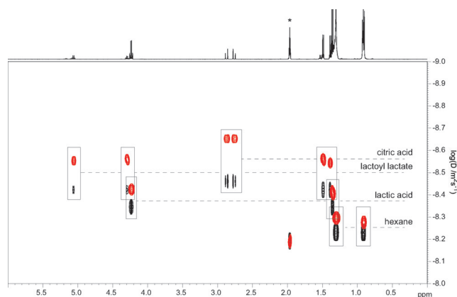
Figure 5. Black and top trace: Solution state DOSY spectrum of 5 mm hexane, citric acid and lactic acid in [\text{D}_3] acetonitrile. Red: same mixture in the presence of silica HMS. The two spectra have been aligned in the diffusion dimension taking the residual solvent signal (in the absence of microspheres, asterisk) as a reference.
